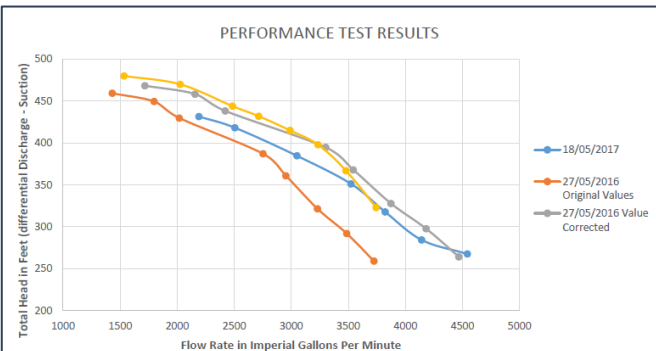
Performance Test for Fire Pump
